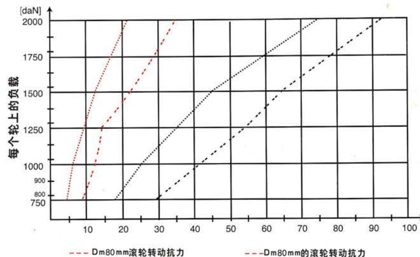
Rotation resistance of the roller of the Dm80mm Dm80mm
